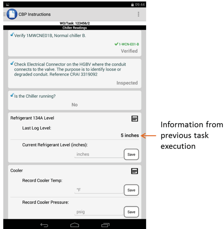
Figure 39. Incorporation of previous log information.
